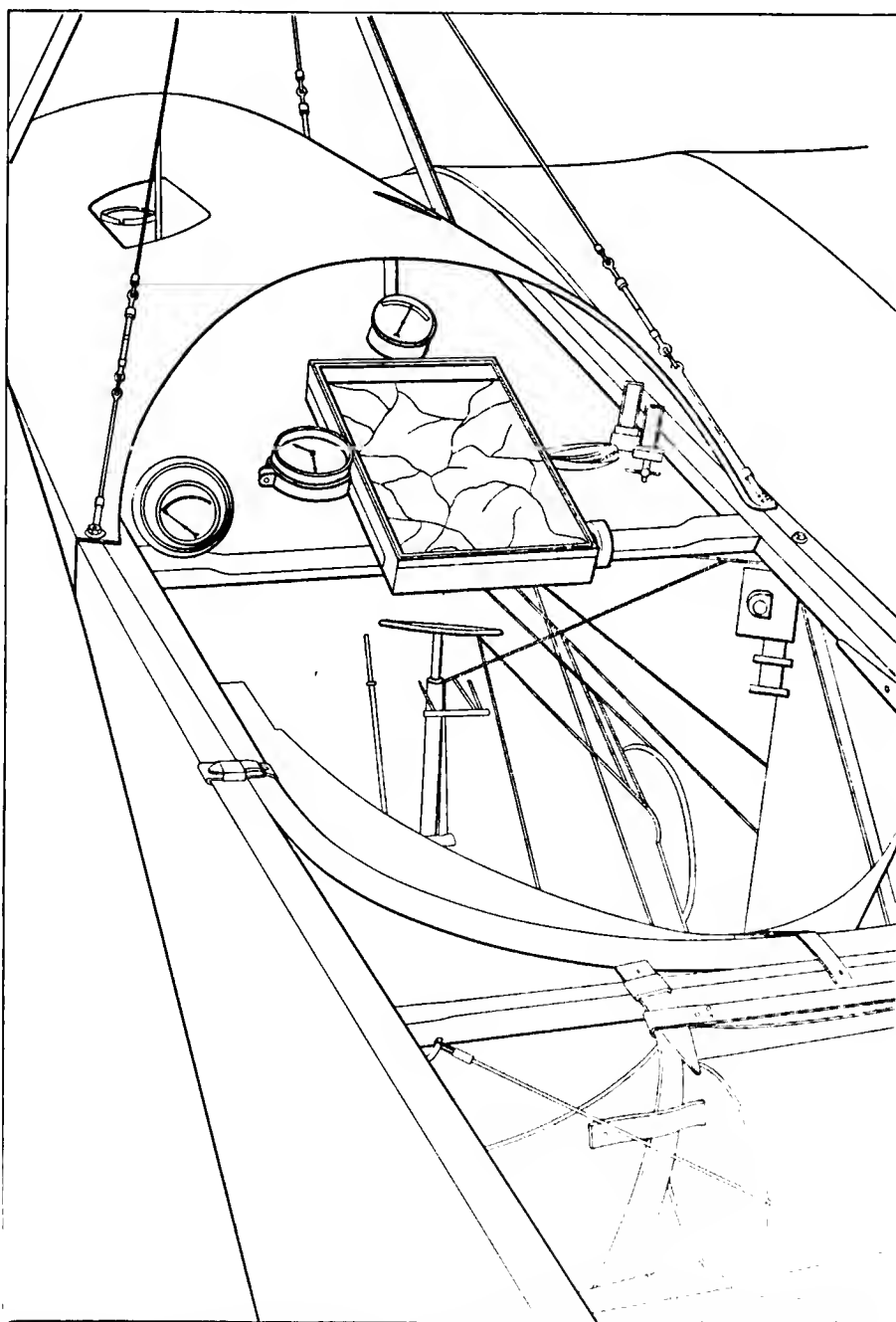
The quarterdeck of a Blériot monoplane. In the center the chart holder; on the right, the compass; above, the barometer; on the left, the clock and the revolutions indicator
